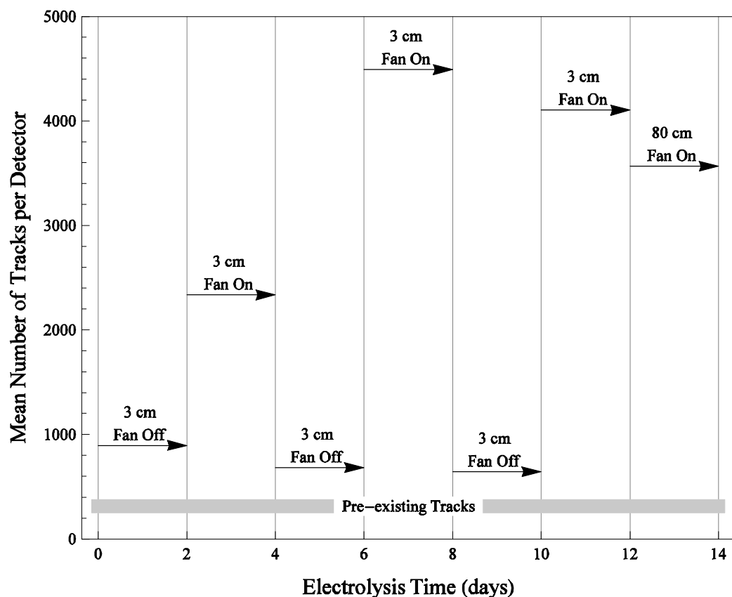
FIGURE 4. Influence of air flow on track density. The experiment consisted of 7 consecutive 2-day runs during which the electrolysis cell remained on. In each run 2 or 3 chips were placed either 3 or 80 cm from the cell, and a fan directed at the chips was either on or off. Track density in excess of background is an order of magnitude greater when the fan is on compared with when it is off, independent of the separation of the chips and the cell.
