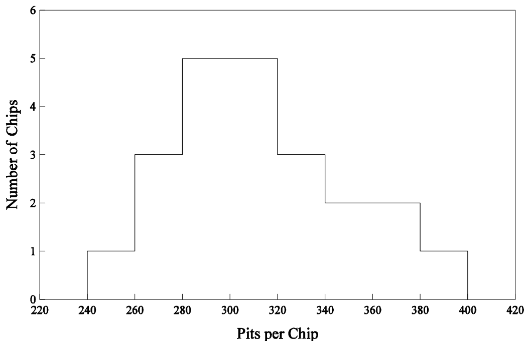
FIGURE 2. Latent tracks in detector chips as received from the manufacturer. The histogram shows the numbers of detector chips having counts in 20-pit intervals from 240 to 400 pits per chip. The mean number of pits per chip is 314.
