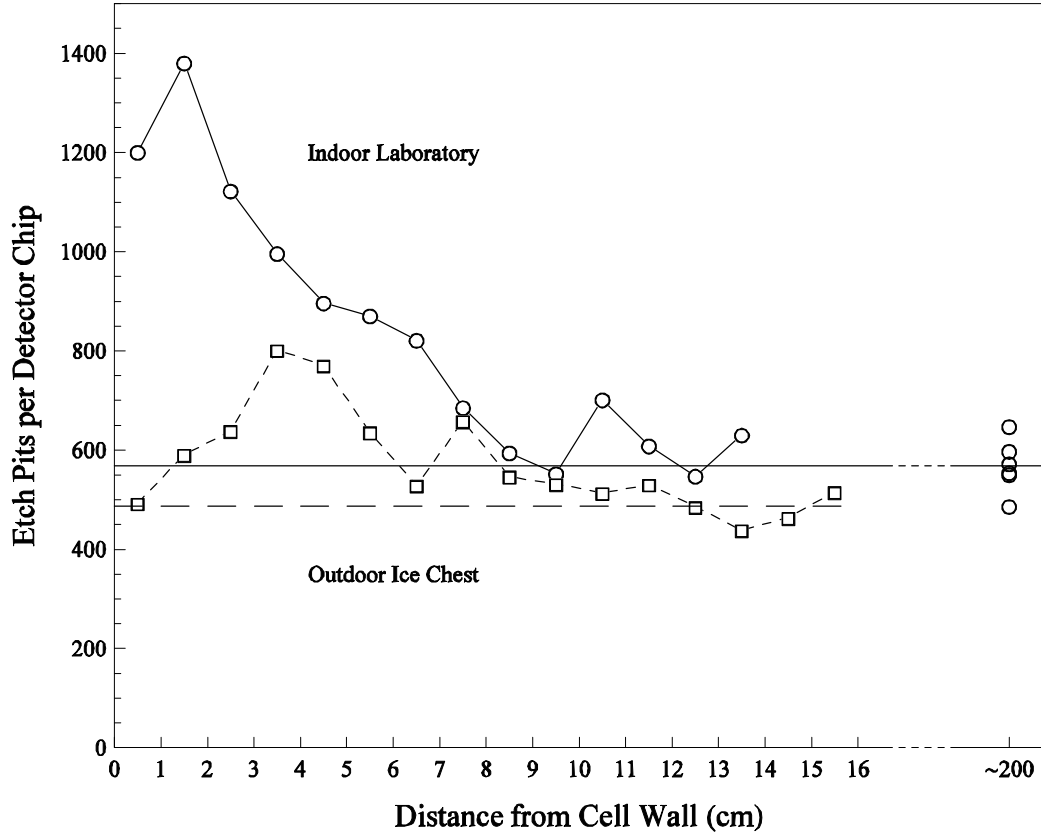
FIGURE 3. Density of etch pits as a function of distance from the cell. Chips measuring 1 cm × 2 cm were placed with long edges in contact on a horizontal surface about 1 cm below the level of the O-ring. Exposures of 4 days were made in an indoor laboratory and in an outdoor ice chest. The indoor exposure suggests that energetic particles may reach out to a distance of about 8 cm from the cell (the solid horizontal line is a background level determined from 6 remote detectors at a distance of about 200 cm). The ice chest exposure suggests a weakened or dead cell as discussed in the text.
