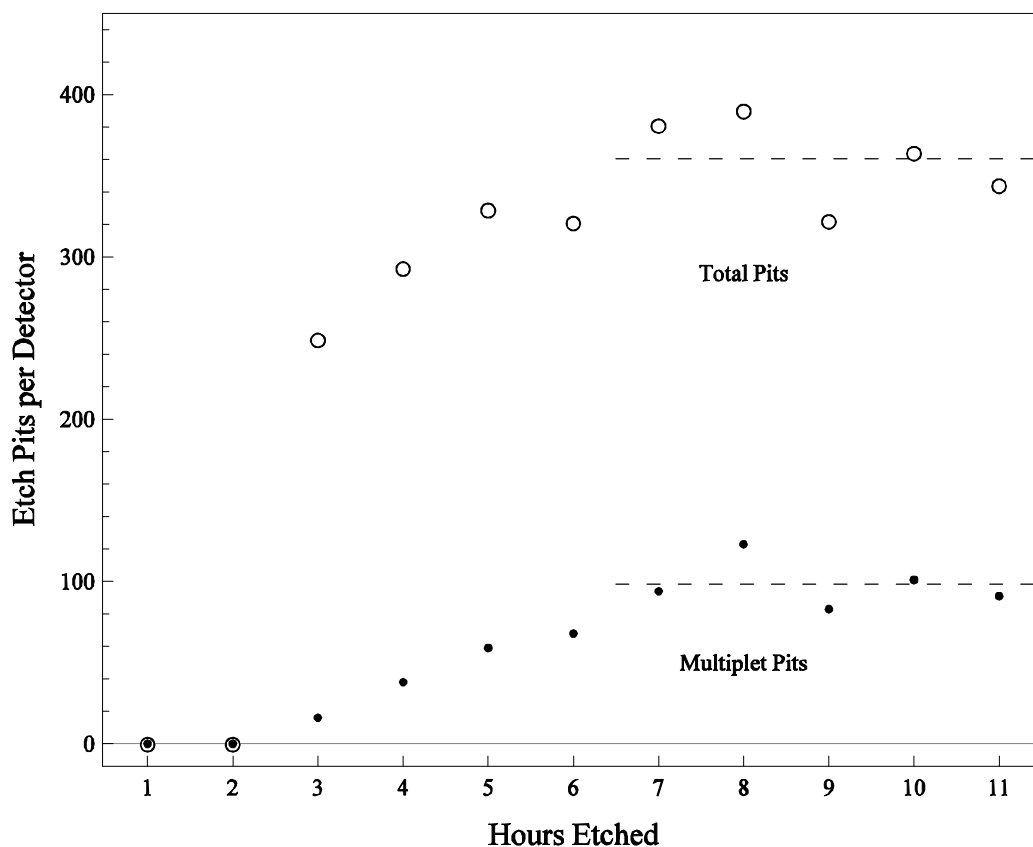
FIGURE 1. Etch pit density as a function of etching time in 6.5N KOH at 80C. Density is measured in etch pits per 1.5 \text{ cm}^2 detector area. Total pits include those that occur in multiplets of 2 or 3 from decay of embedded radon. No pits are formed for etching times of 1 or 2 hours, after which the density of pits rises and levels off after about 7 hours.
